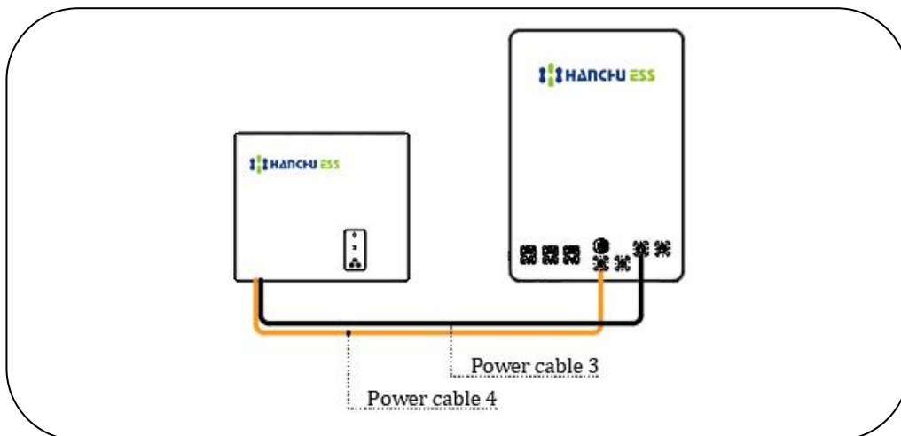
Figure 16 Sample of Power Cable Connection Between the Battery And Inverter
