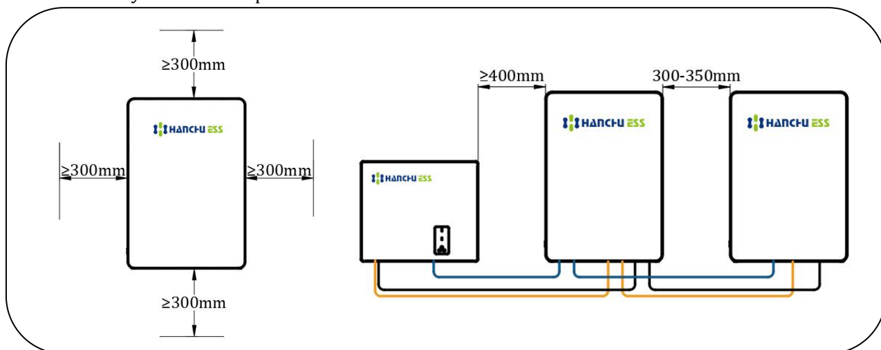
Figure 6 Installation Space
