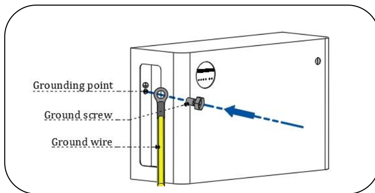
Figure 13 Sample of Battery Ground Connection
